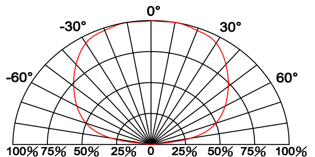
Fig.6 Directive Radiation
